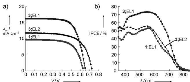
Figure 2. a) Current–voltage curves recorded under AM1.5 conditions and b) IPCE data for DSSCs sensitized with 1 and 3 . Squares (■) and circles (●) represent cells measured with EL1 and EL2, respectively (TiO 2 : 12 \mu\text{m} active and 3 \mu\text{m} scattering layers).
